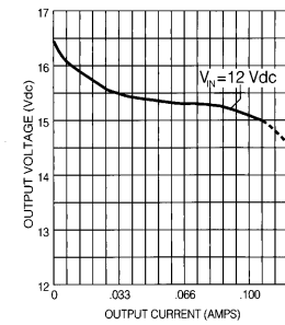
Output Current vs Output Voltage DCH1215D FIGURE 5
