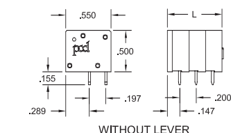
WITHOUT LEVER
