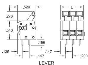
LEVER
