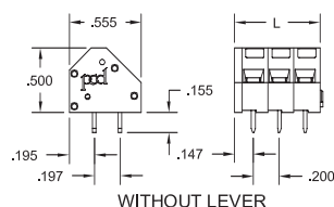
WITHOUT LEVER
