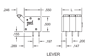
LEVER
