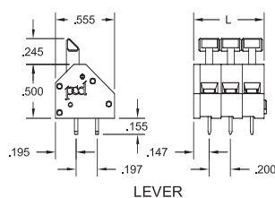
LEVER
