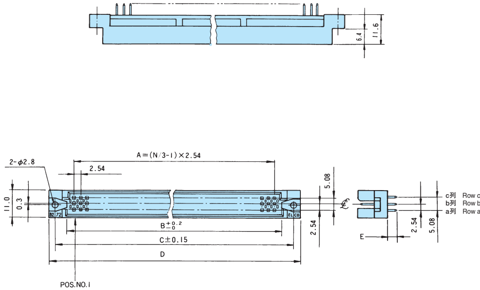
推奨取付寸法 Recommended mounting dimensions
