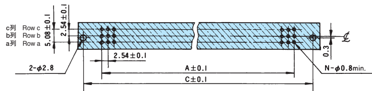
推奨取付寸法 Recommended mounting dimensions
