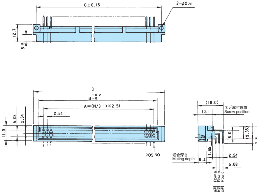
推奨取付寸法 Recommended mounting dimensions
