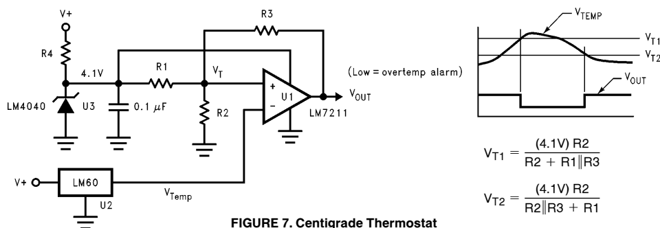
FIGURE 7. Centigrade Thermostat
