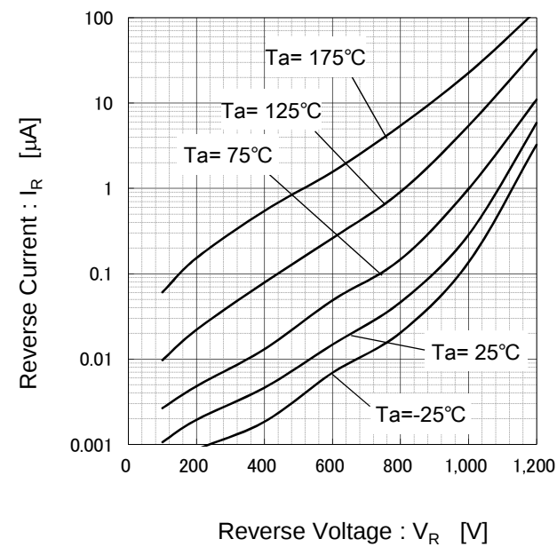
Fig.3 V_R - I_R Characteristics (Per leg)
