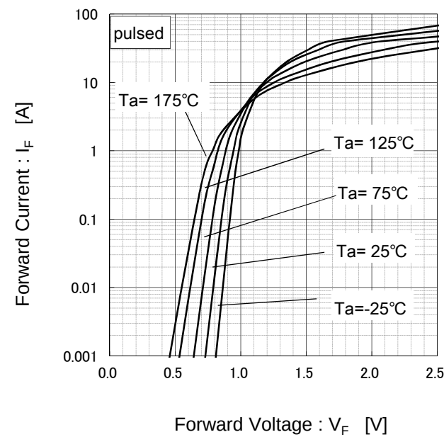
Fig.1 V_F - I_F Characteristics (Per leg)
