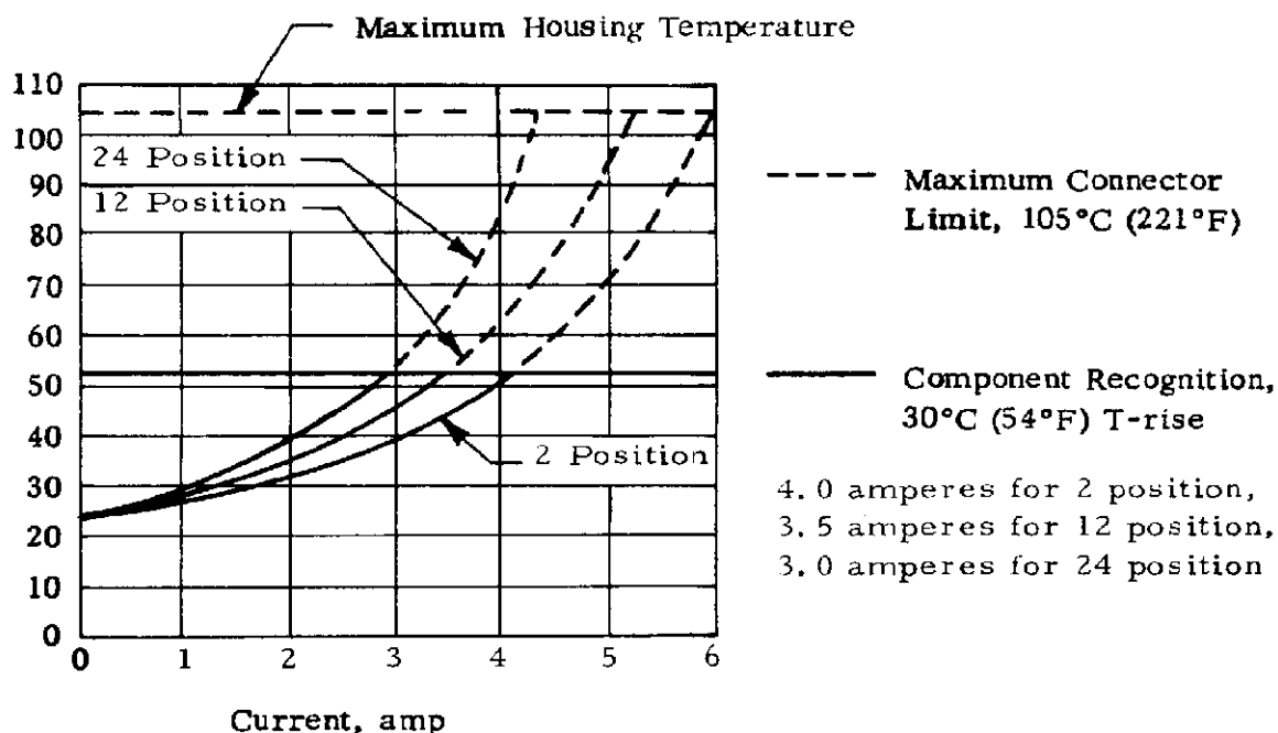
Figure 3 Terminal Temperature vs Current/Circuit 24 AWG Wire
