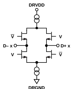
Figure 38. Equivalent Digital Output Circuit
