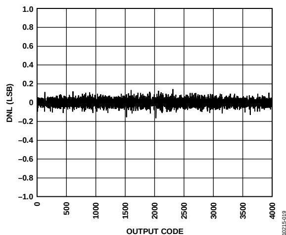
Figure 20. DNL, f_{\text{IN}} = 9.7 \text{ MHz} , f_{\text{SAMPLE}} = 80 \text{ MSPS}
