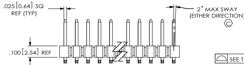
FIG 1 TSM-1XX-XX-XXX-DV SHOWN
