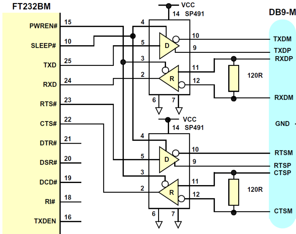
Figure 8.2 USB-RS422 Converter Configuration
