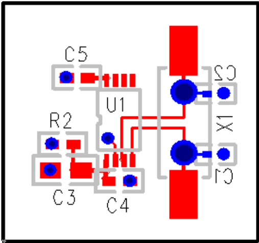
Figure 5B. ICS843051 PC Board Layout Example
