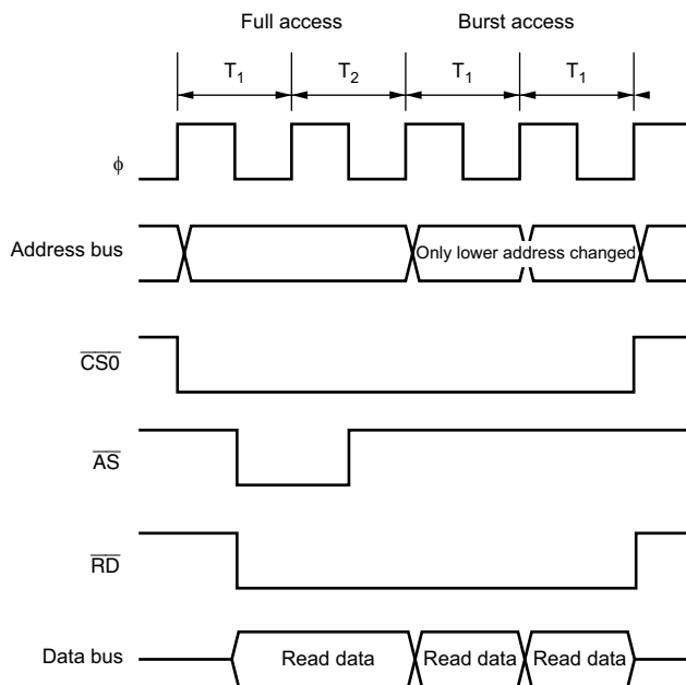
Figure 7.20 Example of Burst ROM Access Timing (When AST0 = BRSTS1 = 0 )
