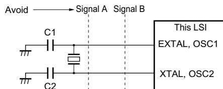
Figure 22.11 Note on Board Design of Oscillator Circuit
