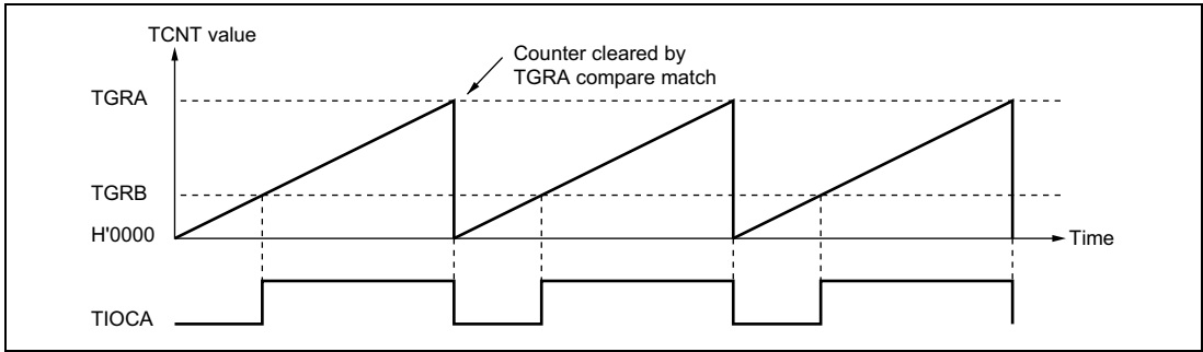
Figure 11.22 Example of PWM Mode Operation (1)
