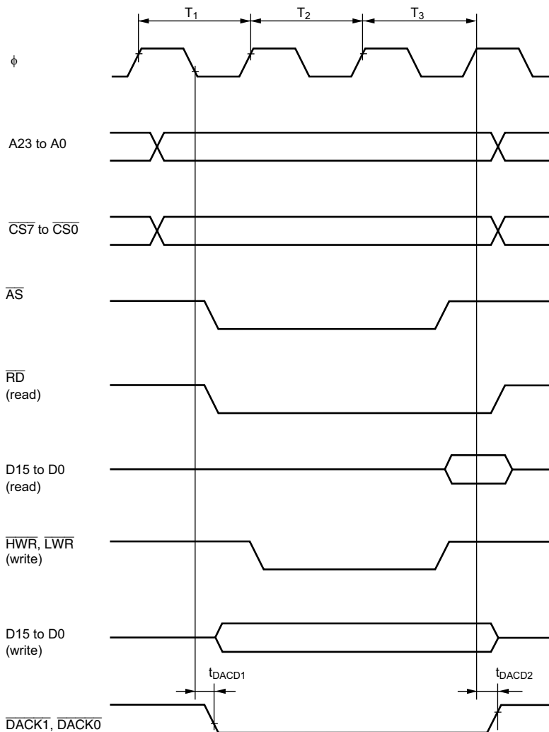
Figure 26.18 DMAC Single Address Transfer Timing (Three-State Access)
