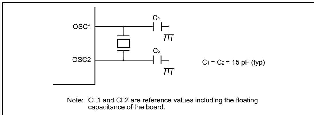
Figure 22.8 Connection Example of 32.768-kHz Quartz Oscillator
