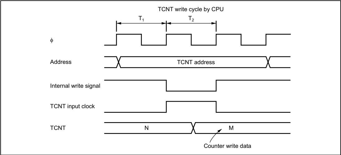
Figure 12.11 Contention between TCNT Write and Increment
