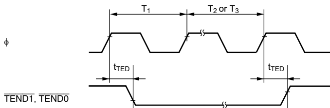
Figure 26.19 DMAC \overline{TEND} Output Timing
