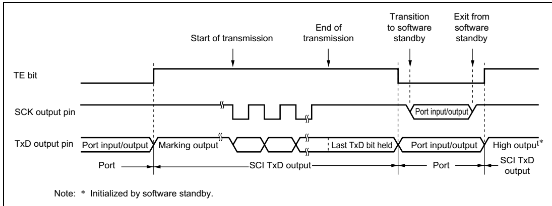
Figure 14.41 Synchronous Transmission Using Internal Clock
