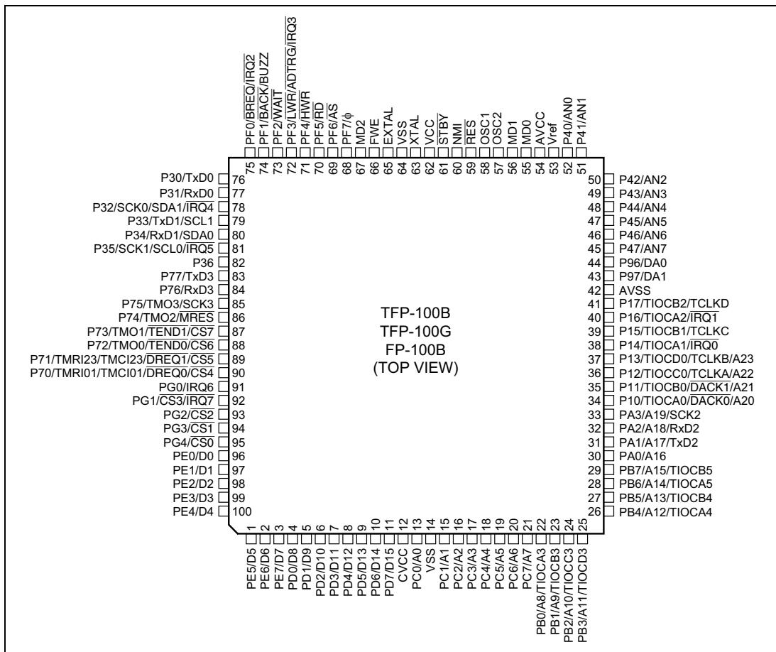
Figure 1.5 Pin Arrangement of H8S/2239 Group (TFP-100B, TFP-100G, FP-100B: Top View)
