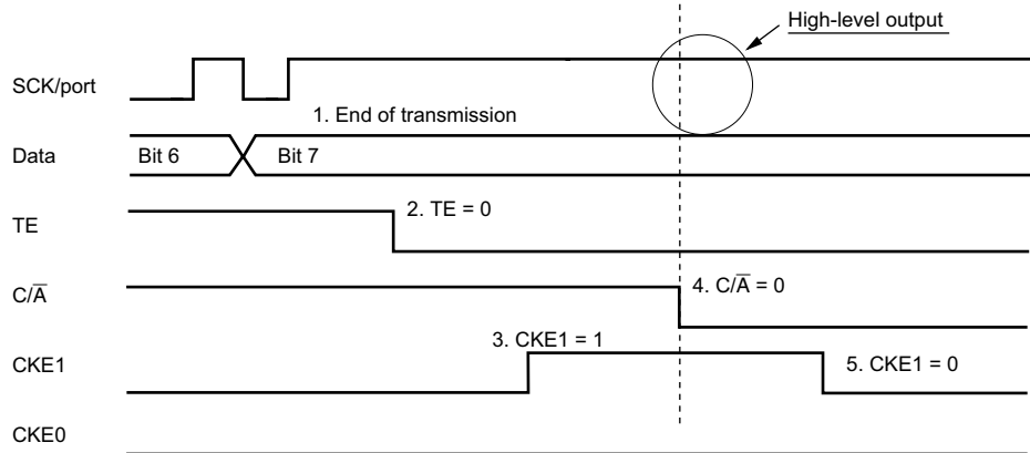
Figure 14.44 Operation when Switching from SCK Pin Function to Port Pin Function (Example of Preventing Low-Level Output)
