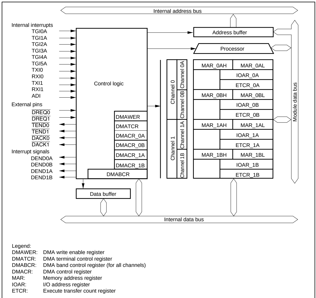
Figure 8.1 Block Diagram of DMAC
