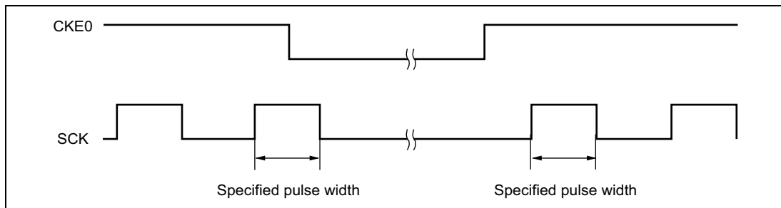
Figure 14.34 Timing for Fixing Clock Output Level
