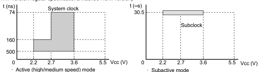
Figure 26.3 Power Supply Voltage and Operating Ranges (H8S/2238 Group)
