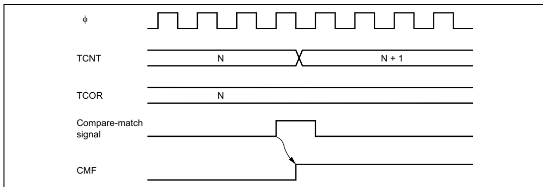
Figure 12.5 Timing of CMF Setting
