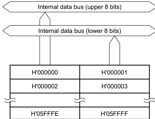
Figure 20.1 Block Diagram of On-Chip Masked ROM (384 kbytes)
