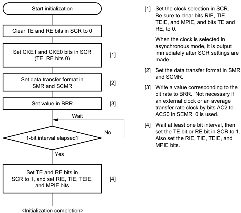
Figure 14.8 Sample SCI Initialization Flowchart
