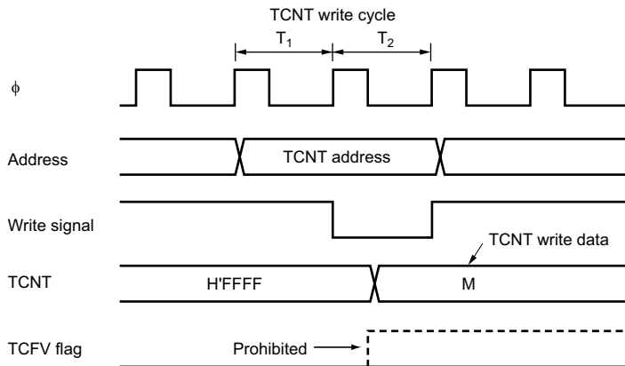
Figure 11.54 Contention between TCNT Write and Overflow
