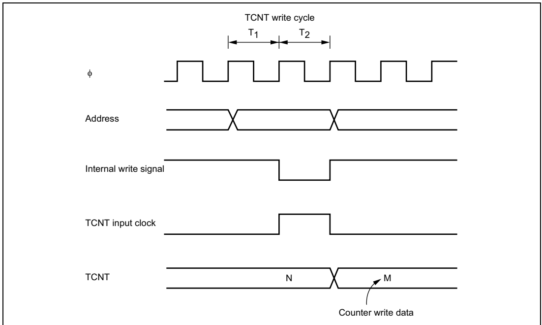
Figure 13.7 Contention between TCNT Write and Increment
