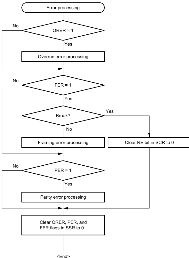
Figure 14.12 Sample Serial Reception Data Flowchart (2)
