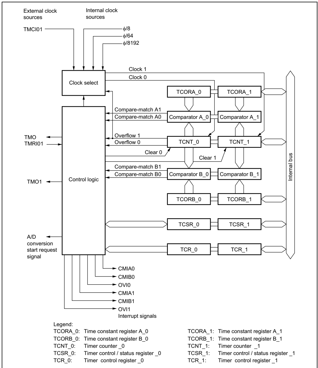
Figure 12.1 Block Diagram of 8-Bit Timer Module
