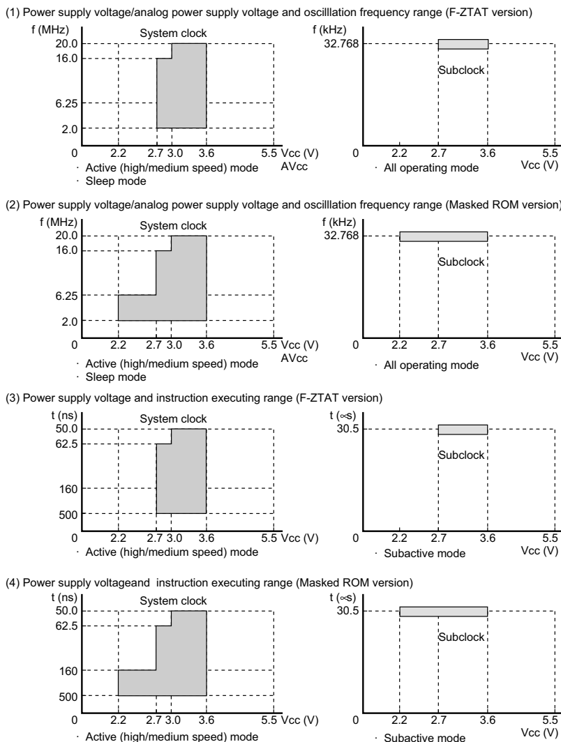
Figure 26.1 Power Supply Voltage and Operating Ranges (H8S/2239 Group)
