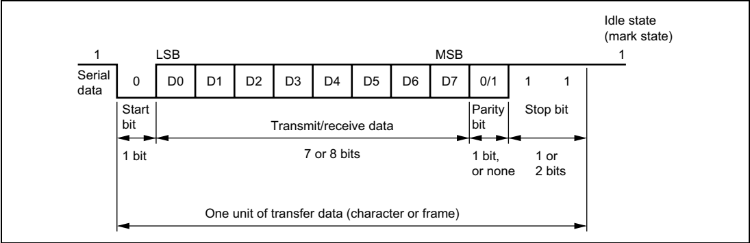
Figure 14.5 Data Format in Asynchronous Communication (Example with 8-Bit Data, Parity, Two Stop Bits)
