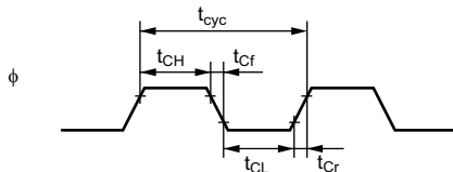
Figure 26.7 System Clock Timing
