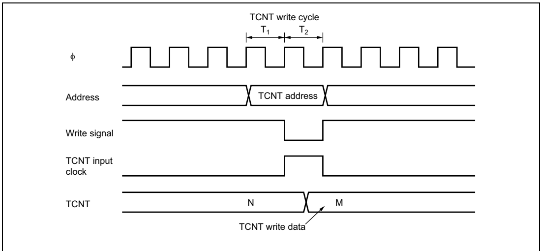
Figure 11.47 Contention between TCNT Write and Increment Operations
