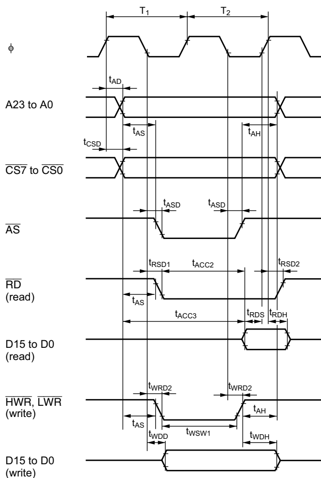
Figure 26.11 Basic Bus Timing (Two-State Access)
