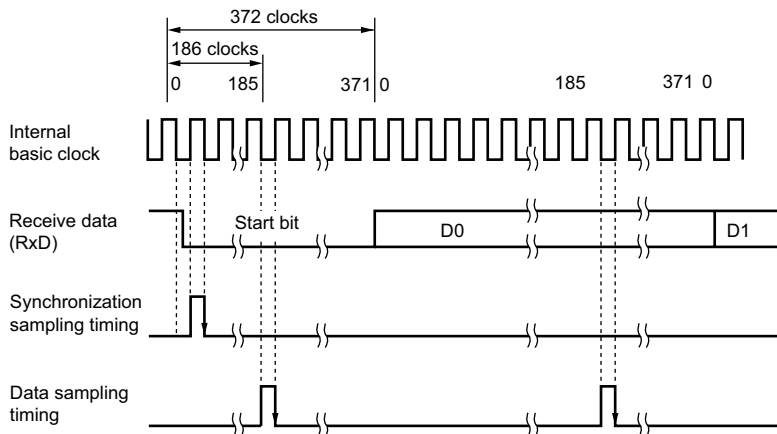
Figure 14.28 Receive Data Sampling Timing in Smart Card Mode (Using Clock of 372 Times the Transfer Rate)
