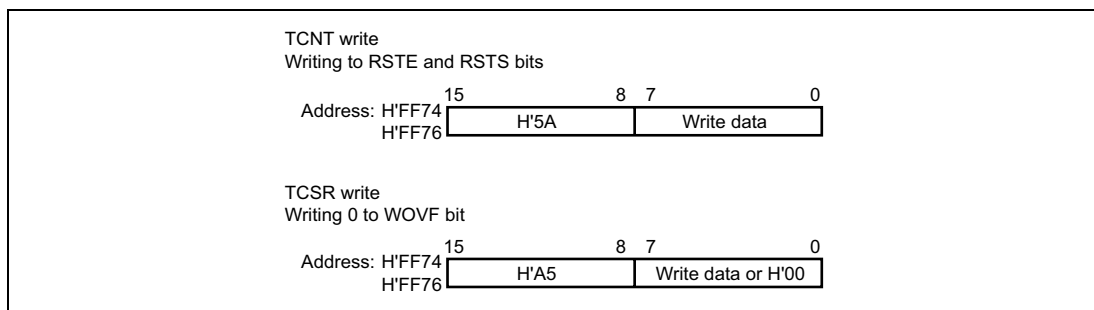
Figure 13.6 Writing to TCNT and TCSR (Example for WDT_0)
