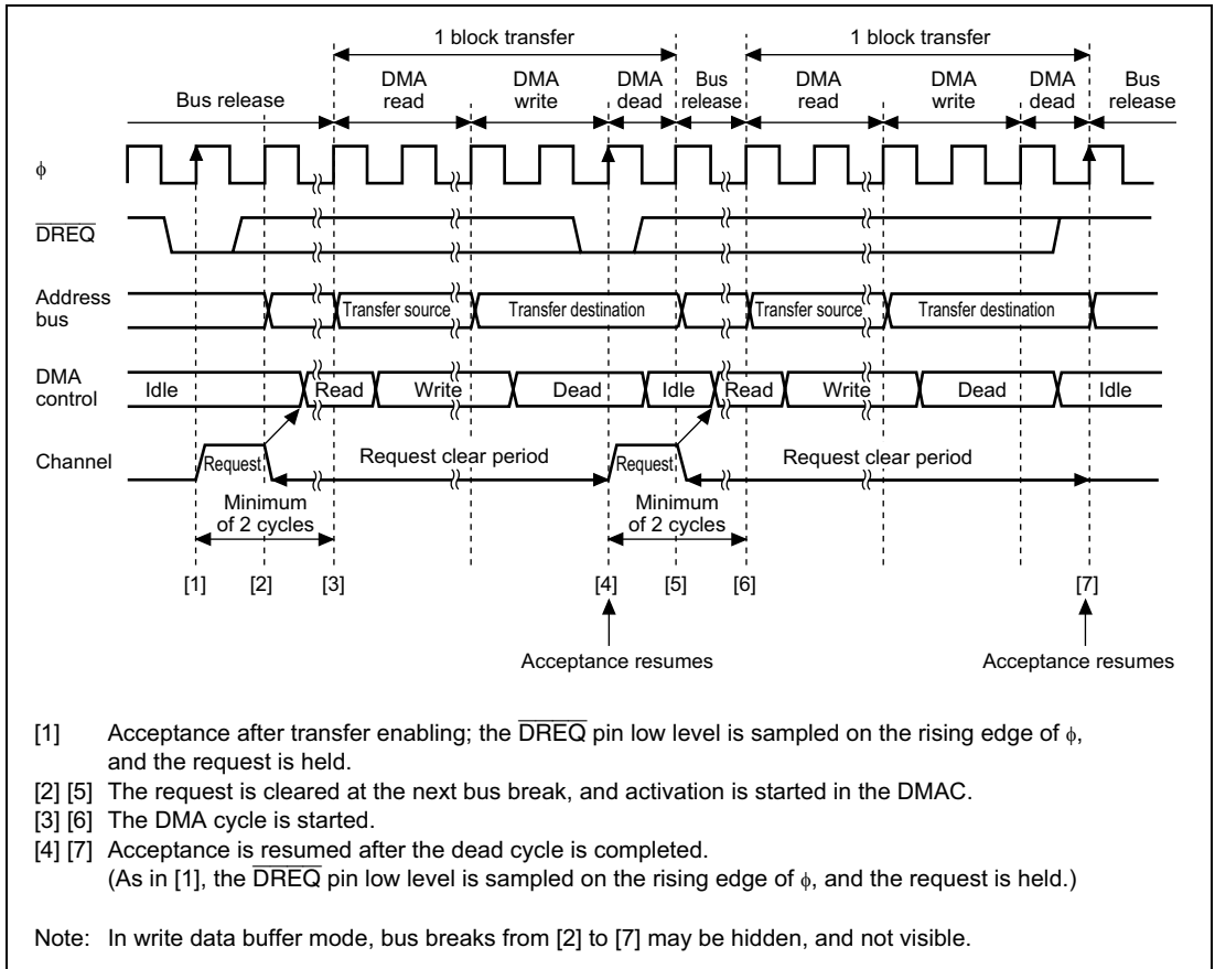
Figure 8.26 Example of \overline{\text{DREQ}} Pin Low Level Activated Block Transfer Mode Transfer
