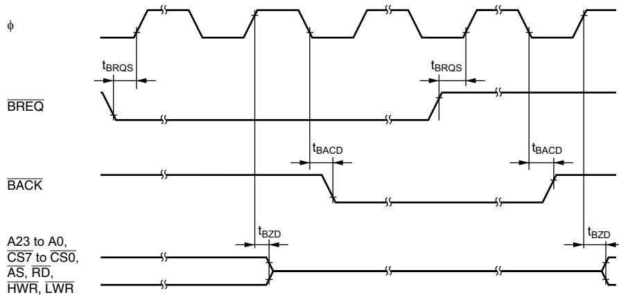
Figure 26.16 External Bus Release Timing
