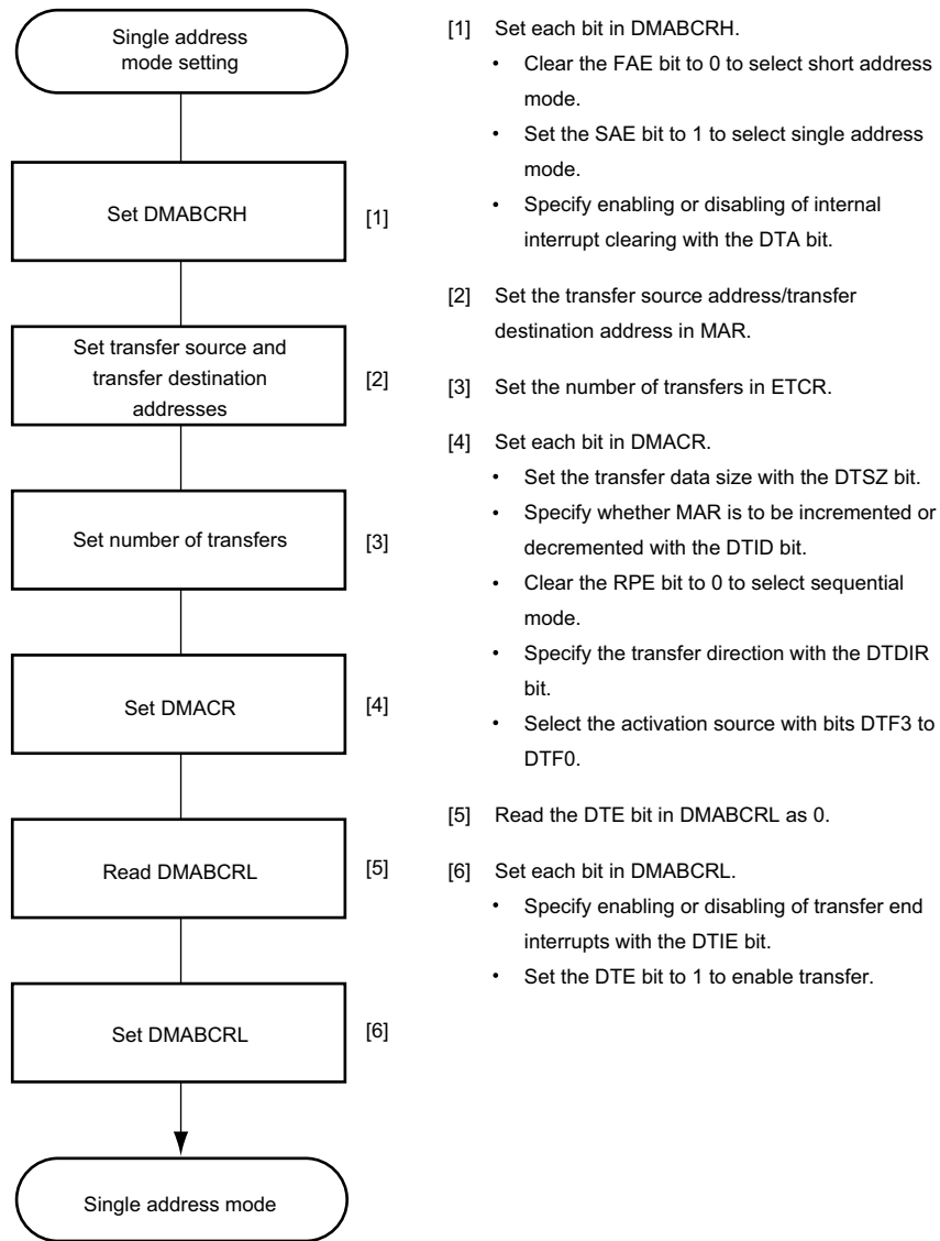
Figure 8.11 Example of Single Address Mode Setting Procedure (When Sequential Mode is Specified)
