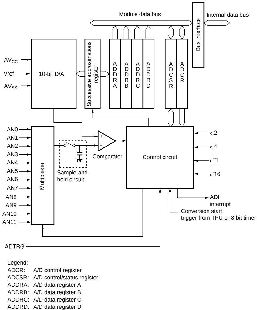
Figure 16.1 Block Diagram of A/D Converter
