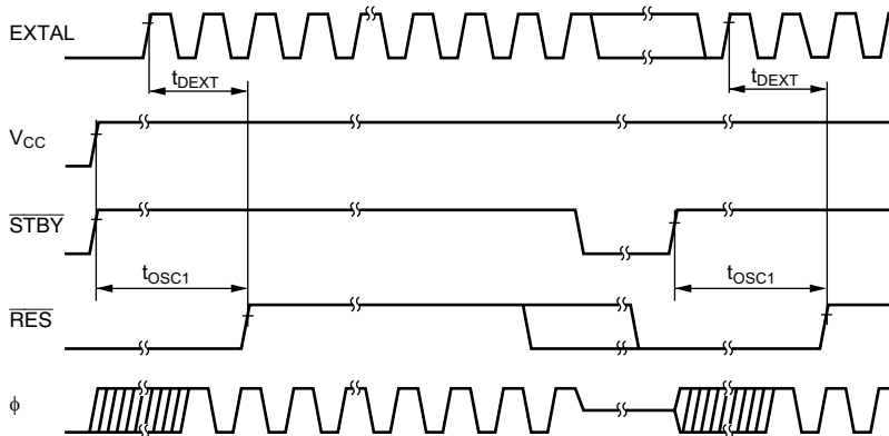
Figure 26.8 Oscillation Stabilization Timing
