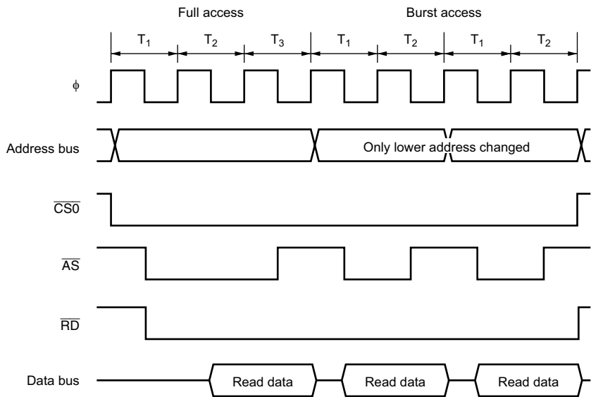
Figure 7.19 Example of Burst ROM Access Timing (When AST0 = BRSTS1 = 1 )
