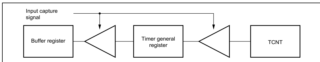
Figure 11.14 Input Capture Buffer Operation
