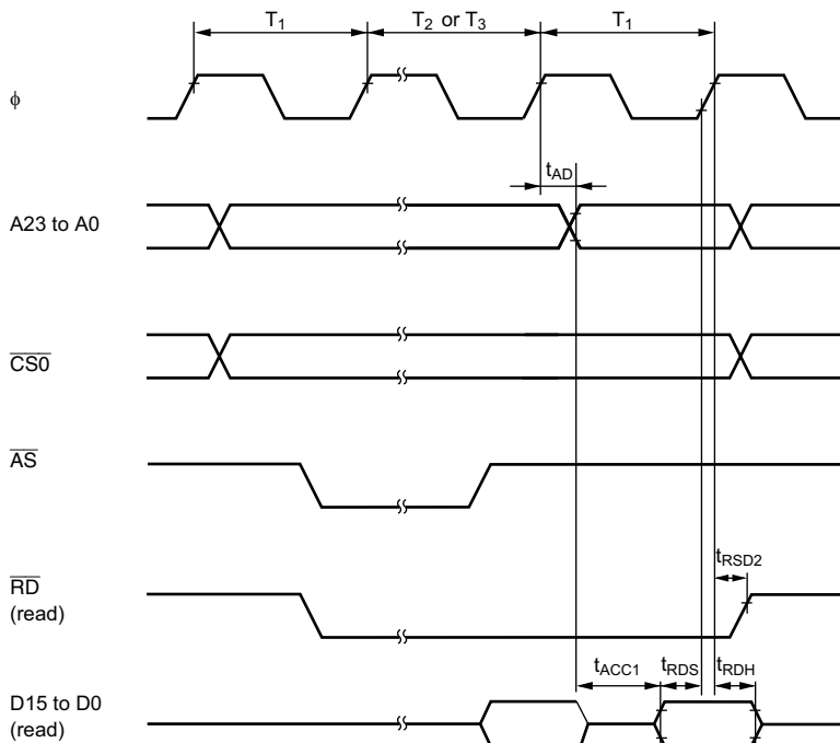
Figure 26.15 Burst ROM Access Timing (One-State Access)
