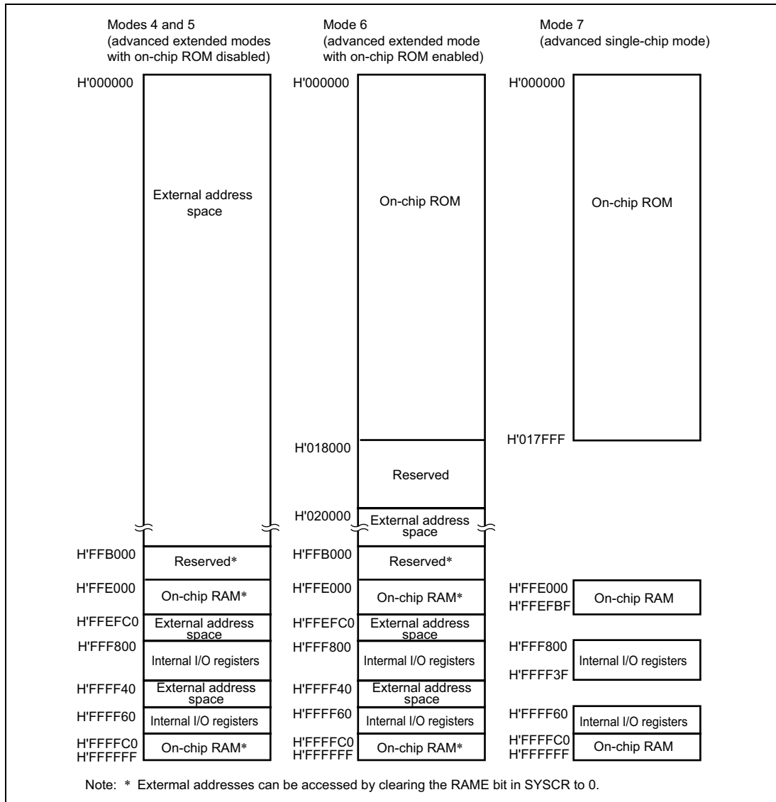
Figure 3.6 H8S/2224 Memory Map in Each Operating Mode
