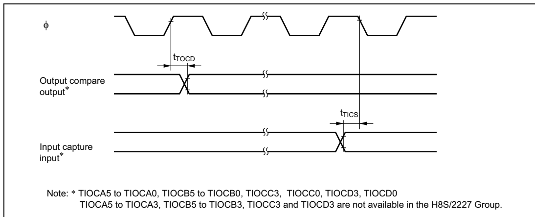
Figure 26.22 TPU Input/Output Timing
