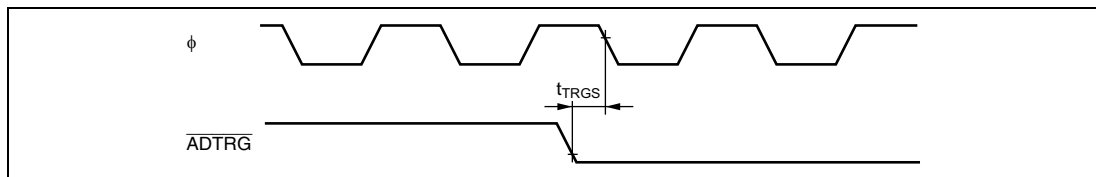
Figure 26.30 A/D Converter External Trigger Input Timing
