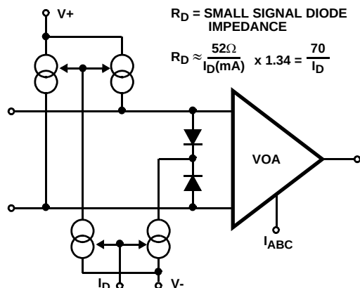
FIGURE 4. VOA SHOWING LINEARIZATION DIODES AND CURRENT DRIVE
