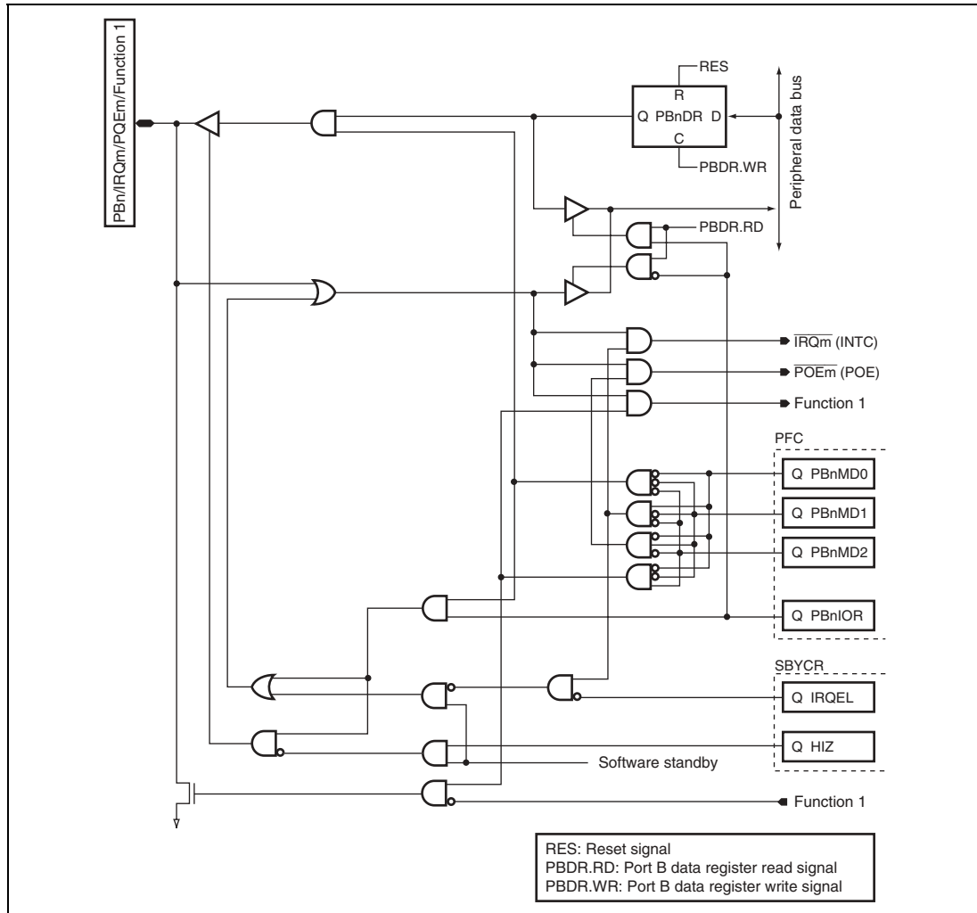
Figure D.15 PBn/IRQm/POEm/Function 1
