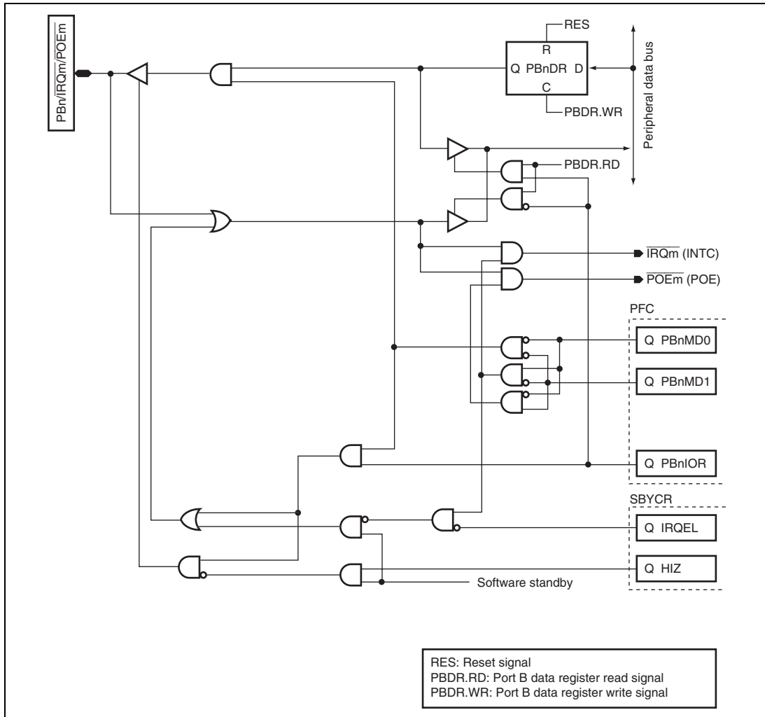
Figure D.16 \overline{\text{PBn/IRQm/POEm}}
