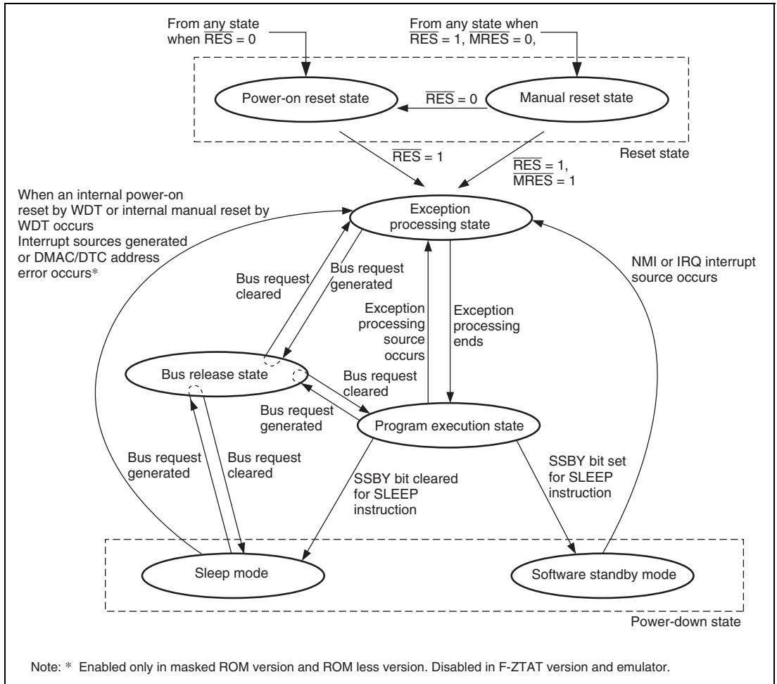
Figure 2.4 Transitions between Processing States
