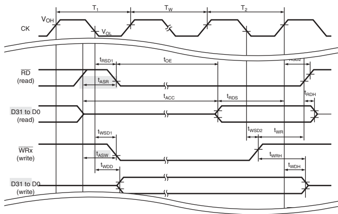
Figure 26.10 Basic Cycle (One Software Wait) 763
