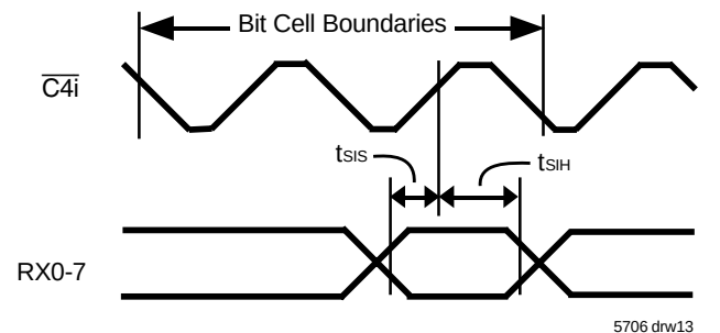
Figure 9. Serial Inputs
