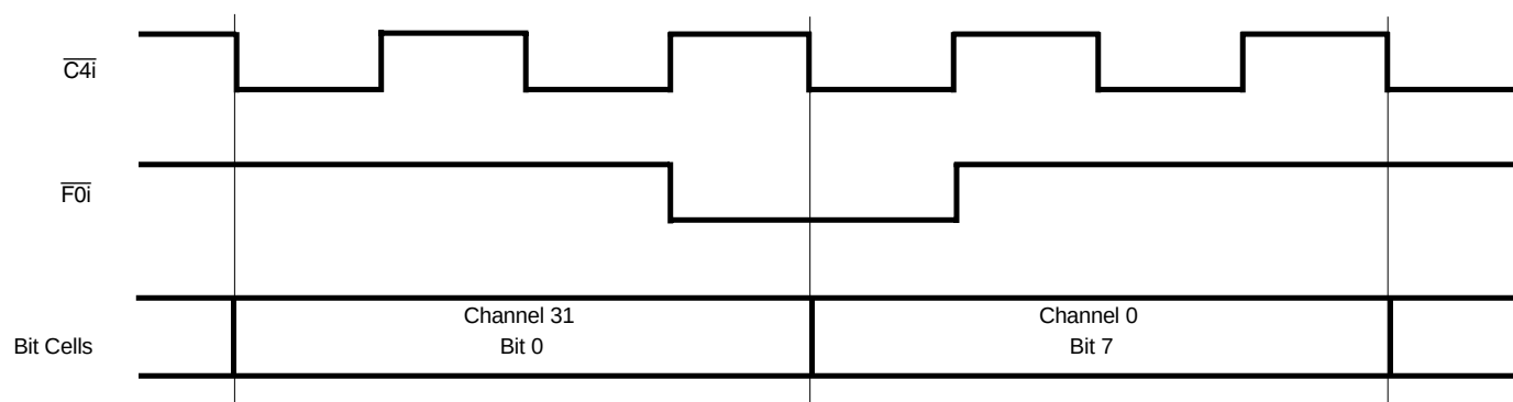
Figure 5. Frame Alignment
