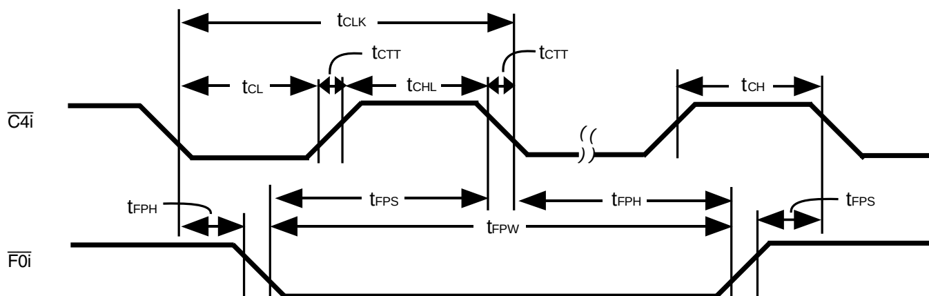
Figure 6. Clock Timing
