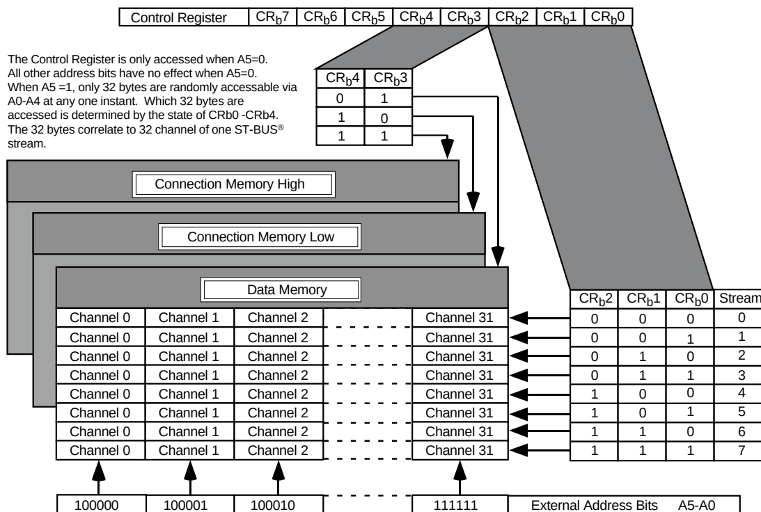
Figure 3. Address Mapping
