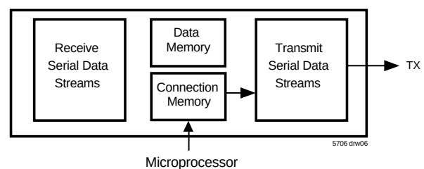
Figure 2. Processor Mode
