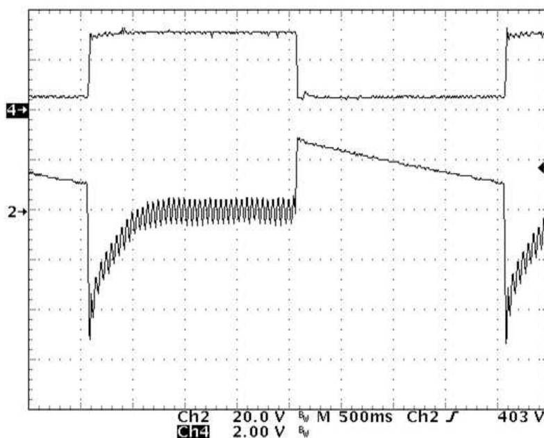
Figure 19. Load Transient
