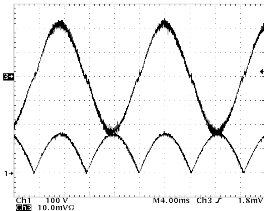
Figure 12. UCC28180EVM-573 Input Current and Input Voltage at the Output of the Bridge Rectifier, (230 V_{AC} , 50 Hz, full load. (CH 1 = rectified input voltage on BR1, 100 V/div., CH 3 = I_{IN} 1 A/div.))
