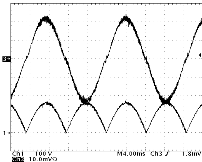
Figure 11. UCC28180EVM-573 Input Current and Input Voltage at the Output of the Bridge Rectifier, (115- V_{AC} , 60 Hz, full load. (CH 1 = rectified input voltage on BR1, 100 V/div., CH 3 = I_{IN} 2 A/div.))
