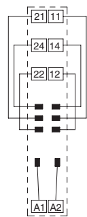
Terminal Arrangement (Top View)
