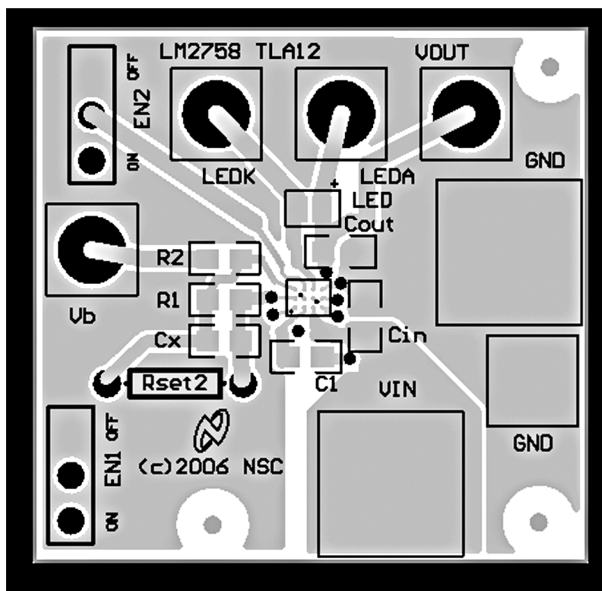
Figure 1. Top Layer
