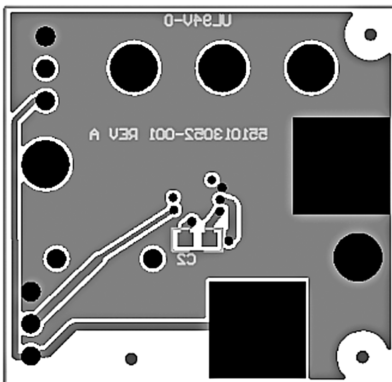
Figure 2. Bottom Layer
