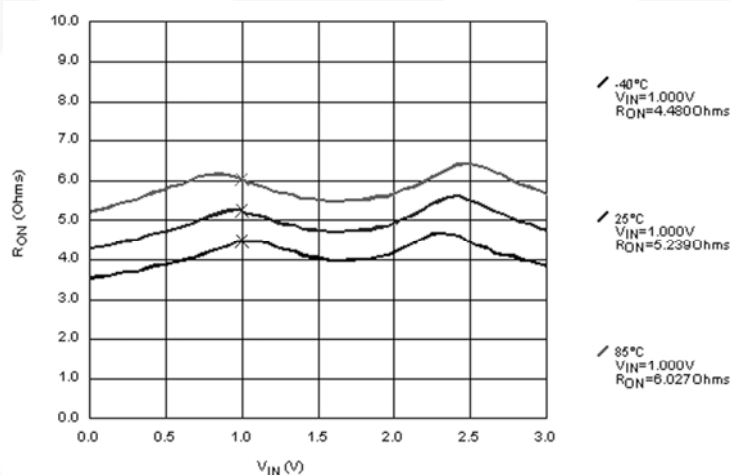
Figure 9. R_{ON} Switch On Resistance, I_{ON}=13mA , V_{CC}=3.0V
