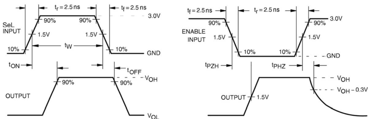
Figure 12. AC Waveforms
