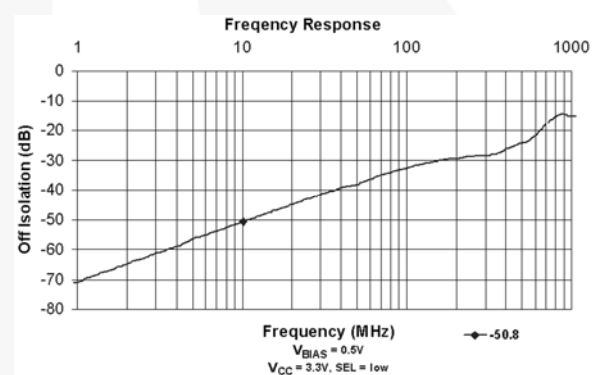
Figure 7. Off Isolation
