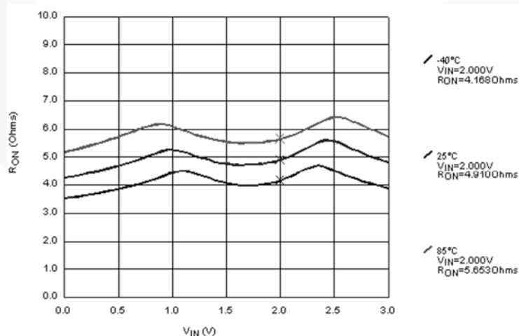
Figure 10. R_{ON} Switch On Resistance, I_{ON}=26mA , V_{CC}=3.0V
