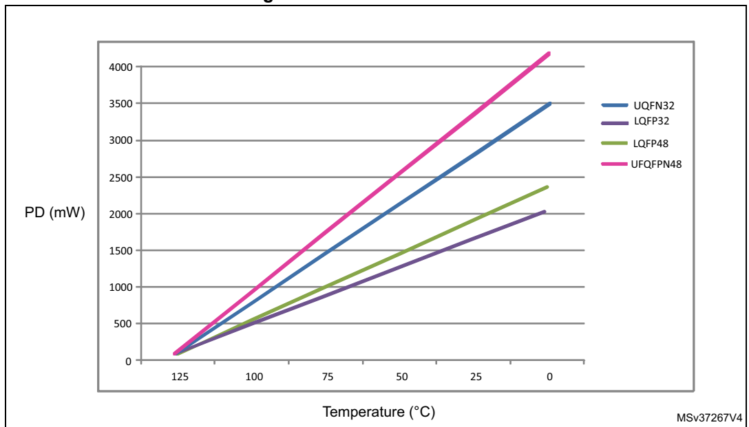
Figure 44. Thermal resistance
