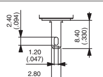
Quick-connect Z1
