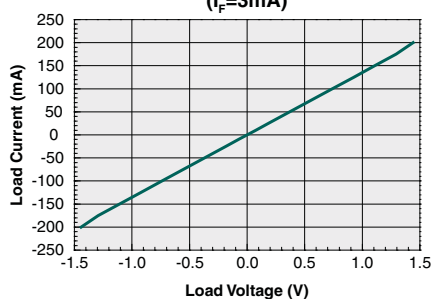
Typical Load Current vs. Load Voltage ( I_F=3\text{mA} )
