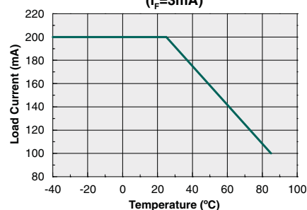
Maximum Load Current vs. Temperature AC/DC Configuration ( I_F=3\text{mA} )
