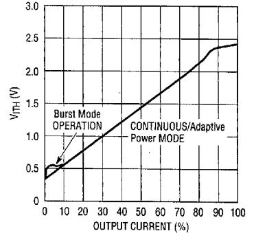
V_{Ith} Pin Voltage vs Output Current
