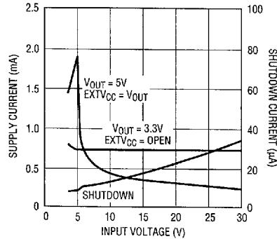
Input Supply Current vs Input Voltage
