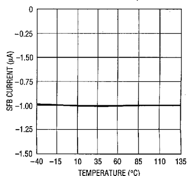
SFB Pin Current vs Temperature
