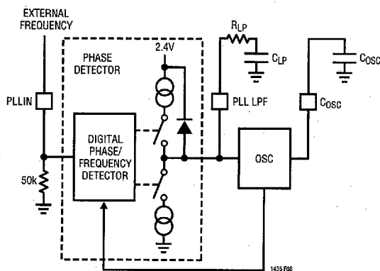
Figure 8. Phase-Locked Loop Block Diagram
