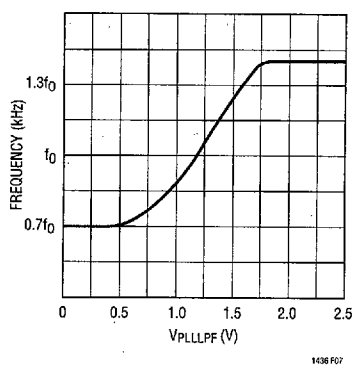
Figure 7. Operating Frequency vs V_{PLL\text{LPF}}
