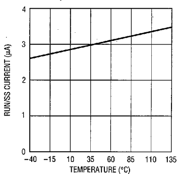
RUN/SS Pin Current vs Temperature
