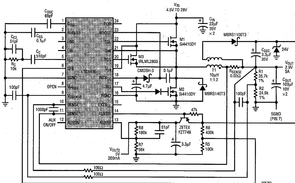
LTC1436 2.9V/5A Adjustable with 5V Auxiliary Output
