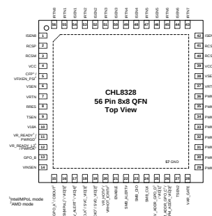
Figure 2: IR3538/CHL8328 Package Top View
