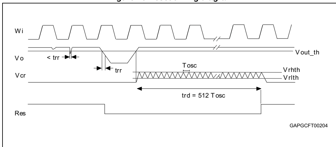
Figure 26.Reset timing diagram
