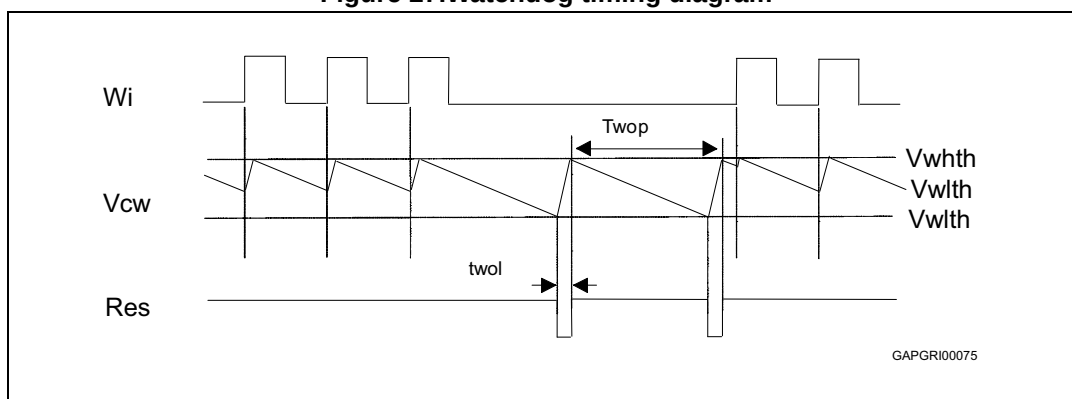
Figure 27.Watchdog timing diagram
