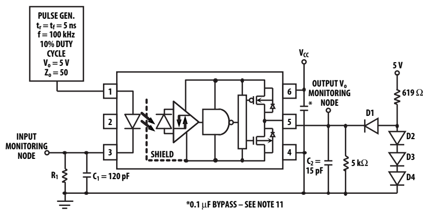
Figure 5. Circuit for t_{PLH} , t_{PHL} , t_r , t_f
