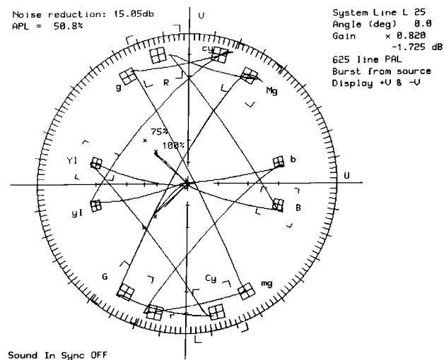
Figure 6. 100% Color Bars on Vector Scope, PAL
