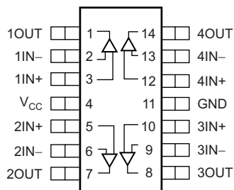
TLV3704 Pin Functions
