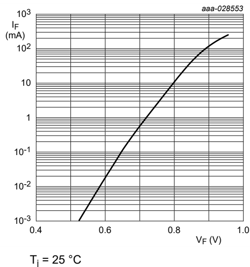
Fig. 5. Forward current as a function of forward voltage; typical values (BZT52H-A/B/C75)
