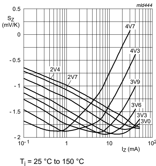
Fig. 6. Temperature coefficient as a function of working current; typical values (BZT52H-A/B/C2V4 to BZT52H-A/B/C4V7)
