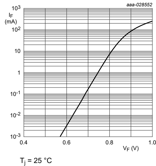
Fig. 4. Forward current as a function of forward voltage; typical values (BZT52H-A/B/C7V5)
