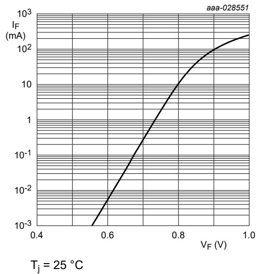
Fig. 3. Forward current as a function of forward voltage; typical values (BZT52H-A/B/C6V8)
