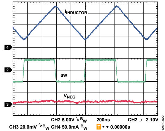
Figure 22. Continuous Conduction Mode Operation Showing Inductor Current ( I_{\text{INDUCTOR}} ), Switch Node Voltage, and Output Ripple, V_{\text{IN}} = 5\text{ V} , V_{\text{NEG}} = -5\text{ V} , I_{\text{LOAD}} = 50\text{ mA} , f_{\text{SW}} = 1.2\text{ MHz} , T_{\text{A}} = 25^{\circ}\text{C}
