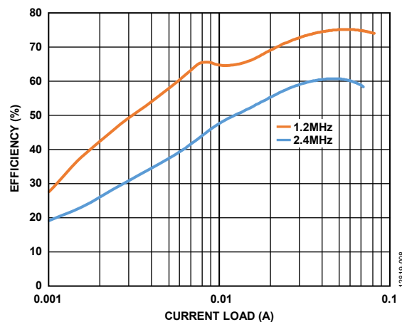
Figure 8. Efficiency vs. Current Load, V_{IN} = 5V , V_{NEG} = -30V , T_A = 25^\circ\text{C}
