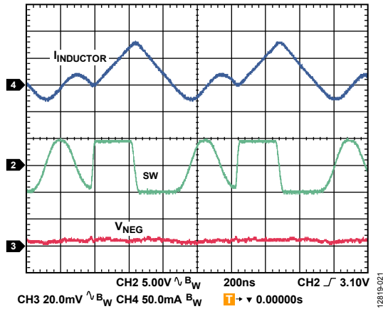
Figure 21. Discontinuous Conduction Mode Operation Showing Inductor Current ( I_{\text{INDUCTOR}} ), Switch Node Voltage, and Output Ripple, V_{\text{IN}} = 5\text{ V} , V_{\text{NEG}} = -5\text{ V} , I_{\text{LOAD}} = 10\text{ mA} , f_{\text{SW}} = 1.2\text{ MHz} , T_{\text{A}} = 25^{\circ}\text{C}
