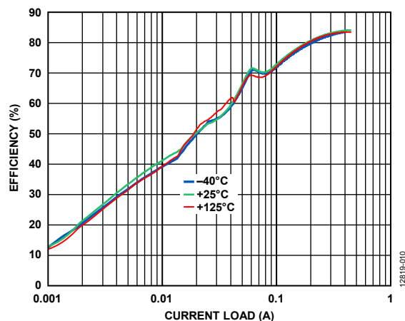
Figure 10. Efficiency vs. Current Load for Various Temperatures, V_{IN} = 5\text{ V} , V_{NEG} = -15\text{ V} , f_{SW} = 1.2\text{ MHz}
