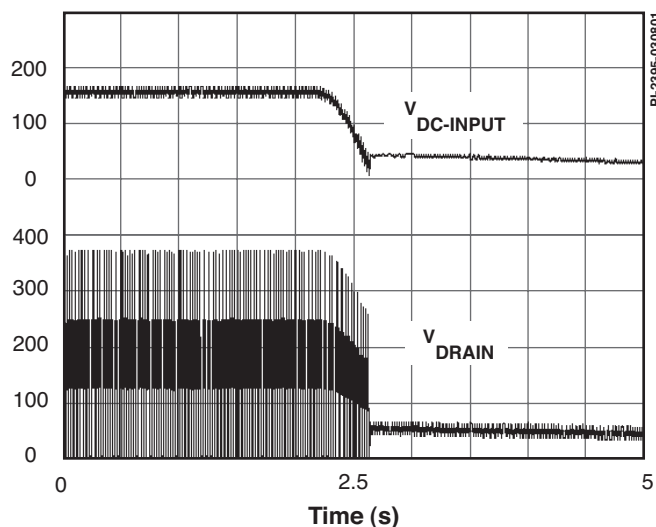
Figure 13. Slow Power-down Timing With Optional External ( 4 \text{ M}\Omega ) UV Resistor Connected to EN/UV Pin.
