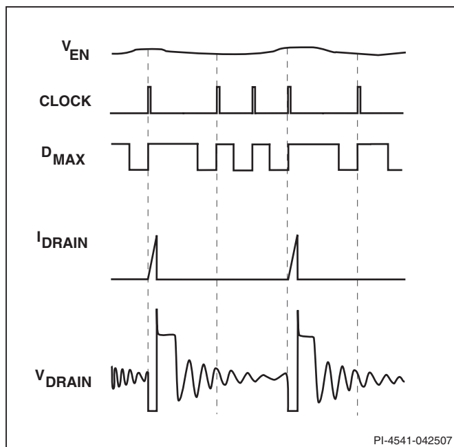
Figure 9. Operation at Very Light Load ( f_{osc} = 132 \text{ kHz} ).
