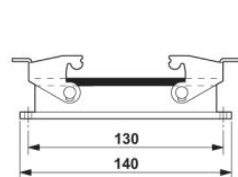
Dimensional drawing
