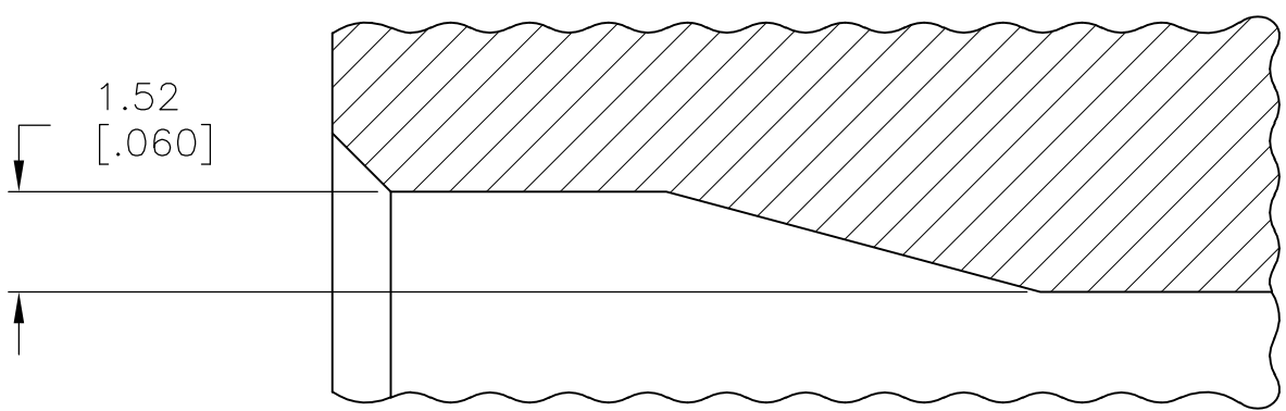
SECTION Z-Z SCALE 8:1
