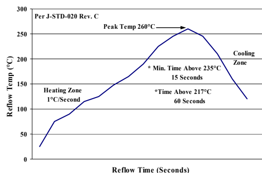
Figure 50. Recommended linear reflow profile using Sn/Ag/Cu solder.
