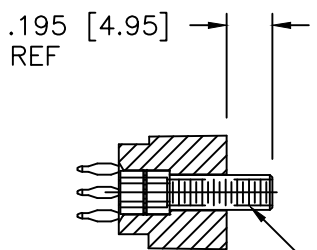
SEC B-B
