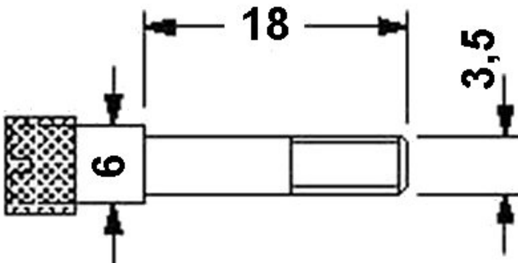
Dimensioned drawing
