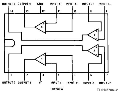
Dual-In-Line Package
