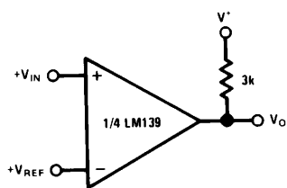
Basic Comparator
