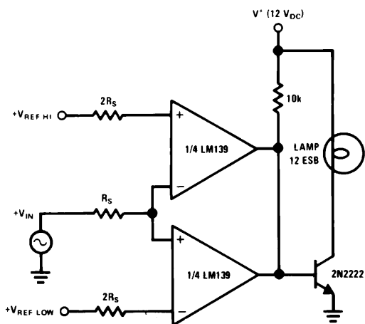
Limit Comparator
