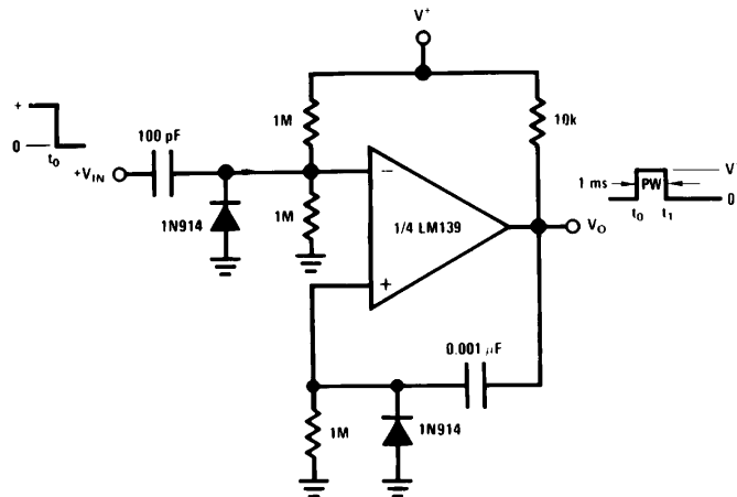
One-Shot Multivibrator
