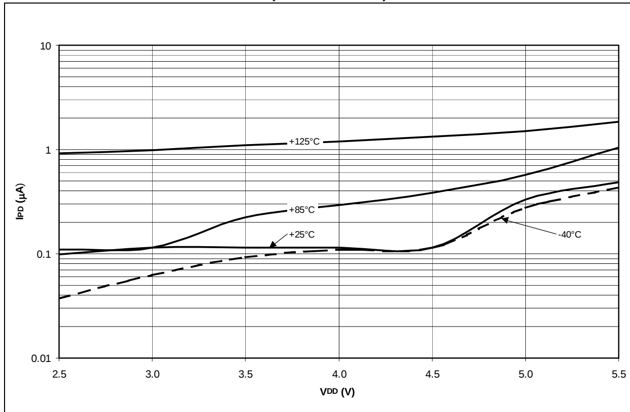
FIGURE 16-18: MAXIMUM I_{PD} VS. V_{DD} ( -40^{\circ}\text{C} TO +125^{\circ}\text{C} )
