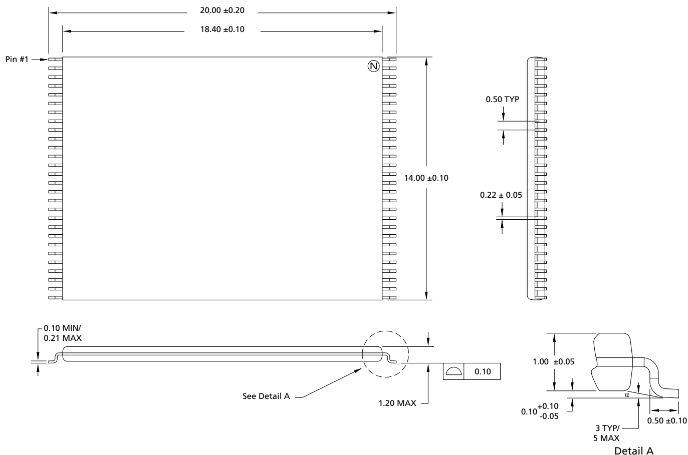
Figure 30: 56-Pin TSOP – 14mm x 20mm
