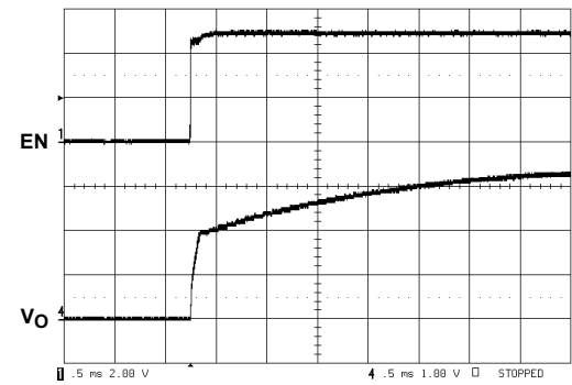
FIGURE 18. RELEASING EN
