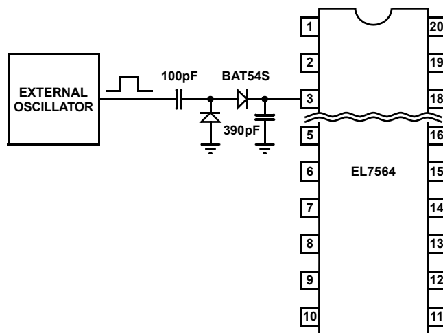
FIGURE 23. OSCILLATOR SYNCHRONIZATION
