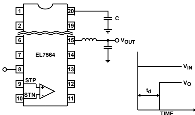
FIGURE 28. START-UP DELAY
