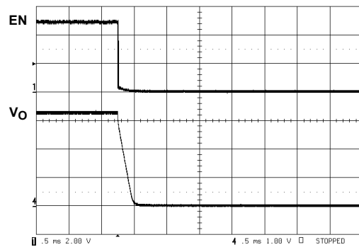
FIGURE 19. SHUT-DOWN
