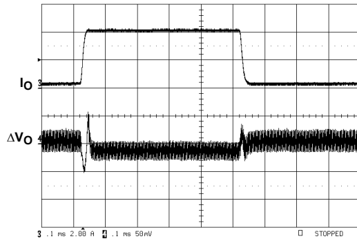
FIGURE 15. TRANSIENT RESPONSE
