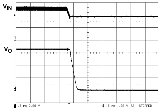
FIGURE 17. POWER-DOWN
