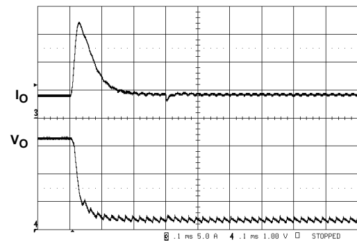
FIGURE 20. SHORT-CIRCUIT PROTECTION
