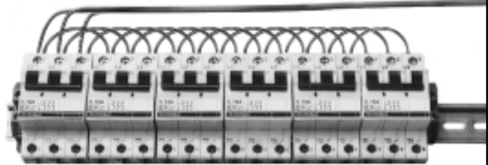
With Busbar
