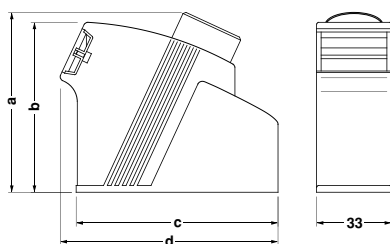
Dimensions: VC-K-T...
