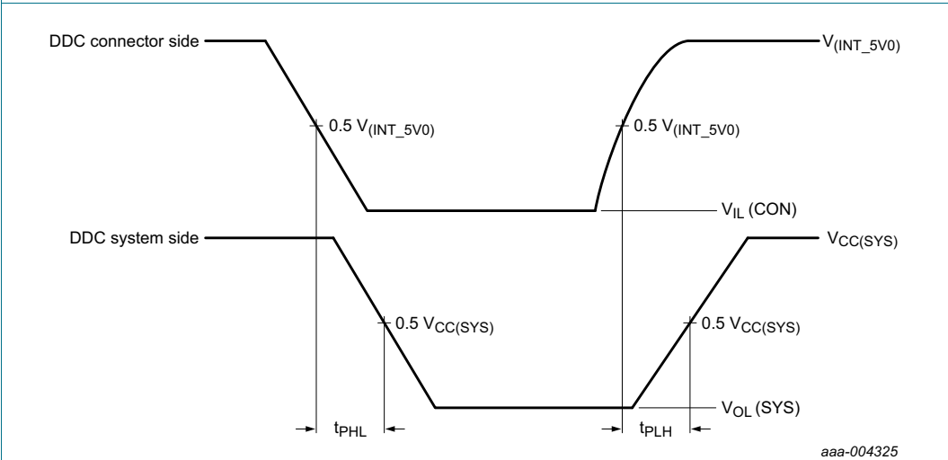
Fig 16. Propagation delay DDC, DDC connector side to DDC system side
