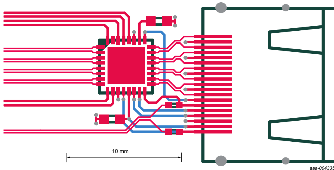
Fig 28. Application of the IP4787CZ32 showing optimized HDMI type-A connector routing
