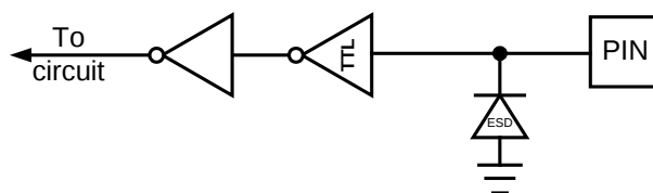
Figure 32: Digital Input Circuit
