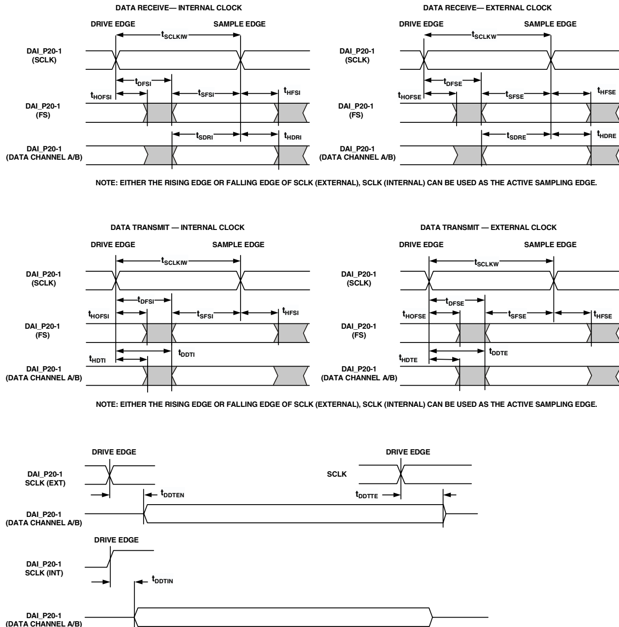
Figure 22. Serial Ports
