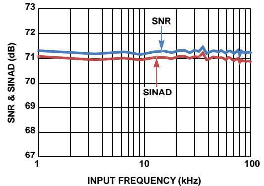
FIGURE 13. SIGNAL-TO-NOISE RATIO AND SIGNAL-TO-(NOISE+DISTORTION) vs INPUT FREQUENCY
