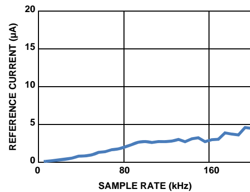
FIGURE 23. REFERENCE CURRENT vs SAMPLE RATE (CODE = FF8h)
