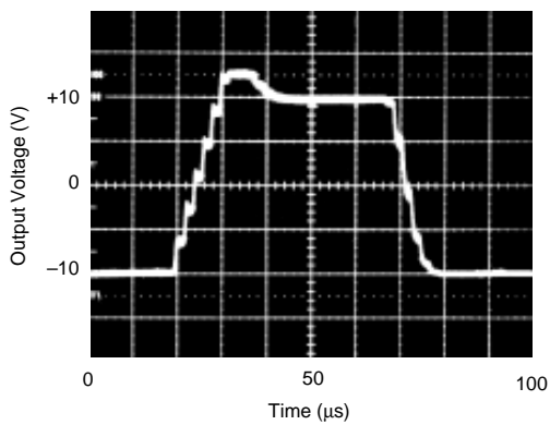
STEP RESPONSE
