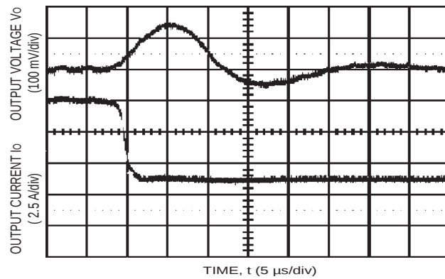
Figure 13. Typical Transient Response to Step Load Change at 2.5 A/ \mu\text{s} from 100% to 50% of I_{O,\text{max}} at 3.3 V Input (COUT = 1 \mu\text{F} ceramic, 10 \mu\text{F} Tantalum).
