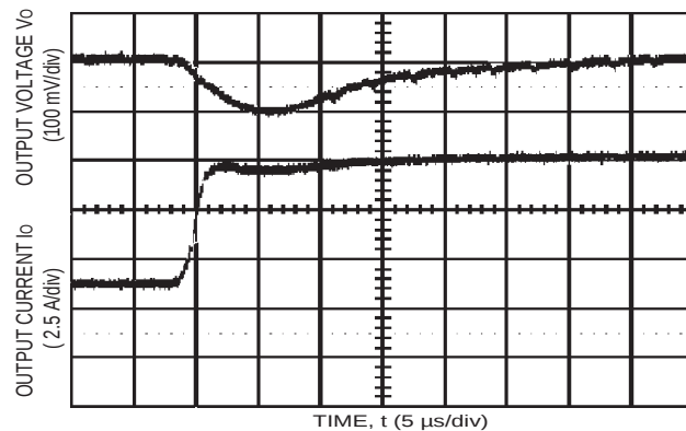
Figure 14. Typical Transient Response to Step Load Change at 2.5 A/ \mu\text{s} from 50% to 100% of I_{O,\text{max}} at 3.3 V Input (COUT = 1 \mu\text{F} ceramic, 10 \mu\text{F} Tantalum).
