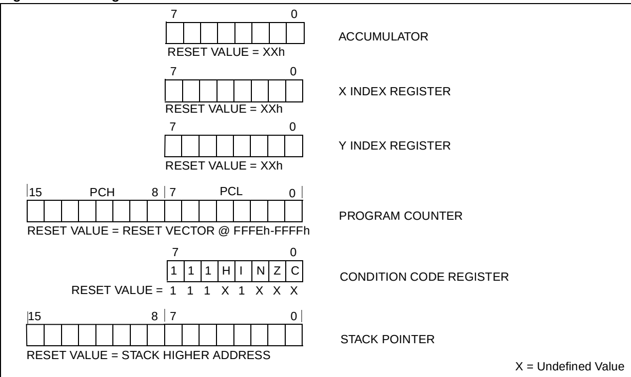
Figure 8. CPU Registers
