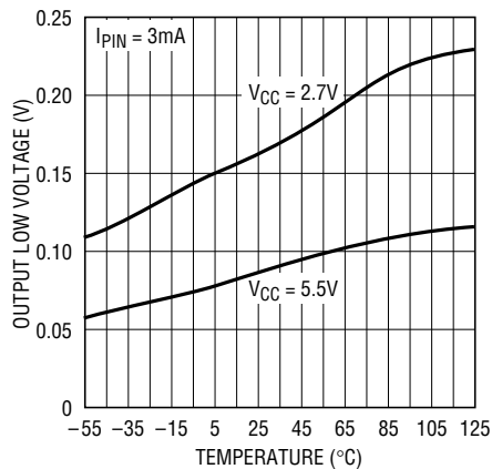
SDA, CPUON, PGTM Output Low Voltage vs Temperature
