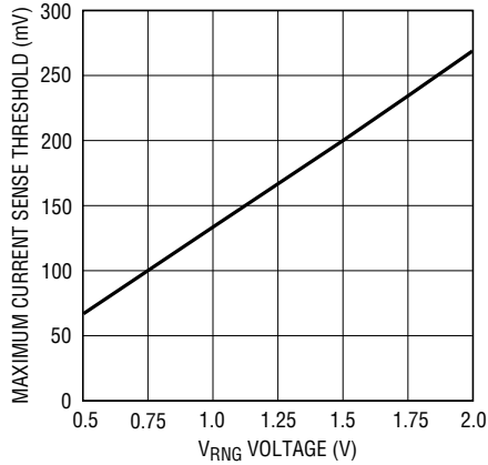
Maximum Current Sense Threshold vs V_{\text{RNG}} Voltage
