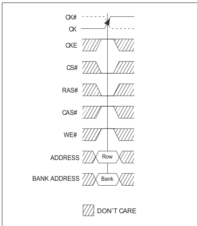
FIGURE 10 - ACTIVE COMMAND
