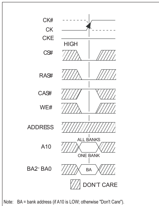
FIGURE 13 – PRECHARGE COMMAND
